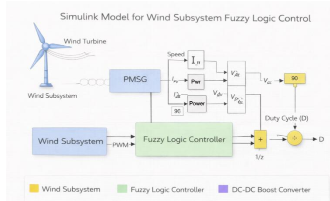
Figure 9. Simulink Model for Wind Subsystem Fuzzy Logic Control
