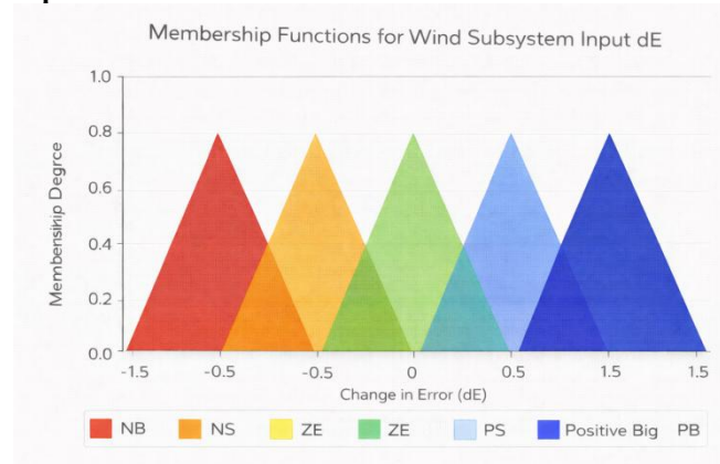
Figure 7. Membership Functions for Wind Subsystem Input dE
