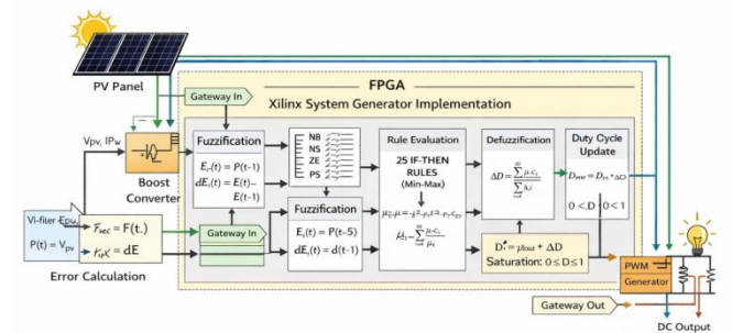
Figure 11: XSG-Based Solar Fuzzy Logic (FL) MPPT Controller Design.
