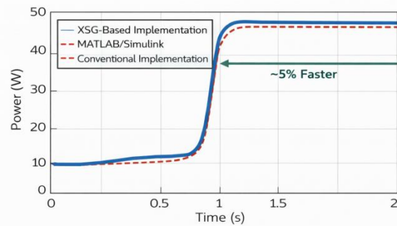
Figure 14: Comparative Power Response of XSG-Based FPGA MPPT Fuzzy Logic Controller and Conventional MATLAB/Simulink MPPT implementation.
