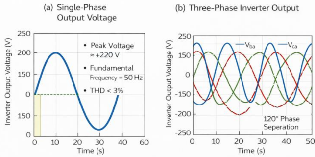
Figure 15: Inverter Output Voltages under Fuzzy Logic-Based Controller, (a) Single-Phase Output Voltage, (b) Three-Phase Output Voltages.
