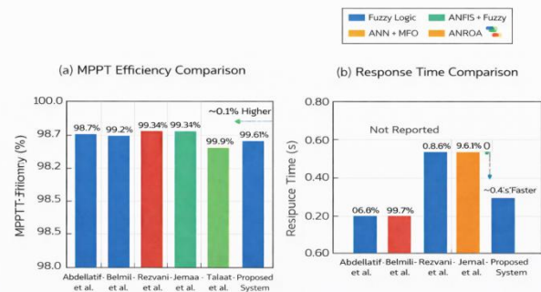
Figure 18: Performance Comparison of the Proposed FPGA-Based System with Previous Studies
