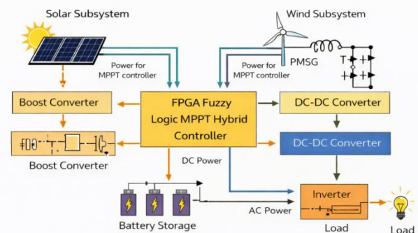
Figure 19: Functional Flow Diagram of the FPGA-Based Fuzzy Logic MPPT Hybrid
