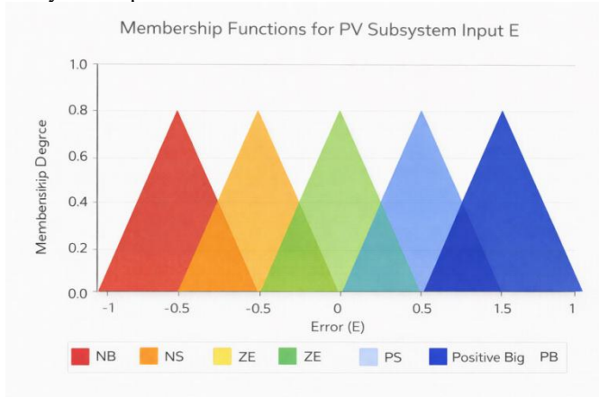
Figure 4. Membership Functions for PV Subsystem Input E
