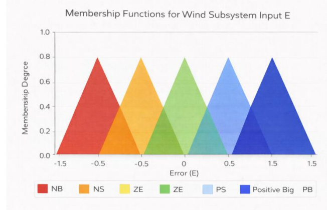
Figure 6. Membership Functions for Wind Subsystem Input E
