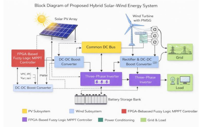
Figure 3. Block Diagram of Proposed Hybrid Solar-Wind Energy System
