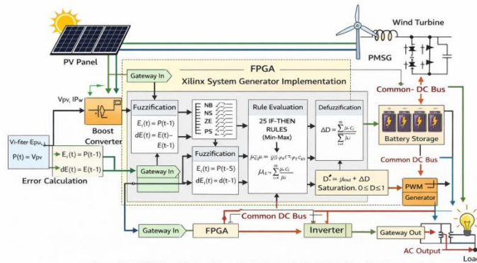
Figure 12: FPGA-Based Optimal Fuzzy Logic Controller for Hybrid Solar-Wind Energy Systems.
