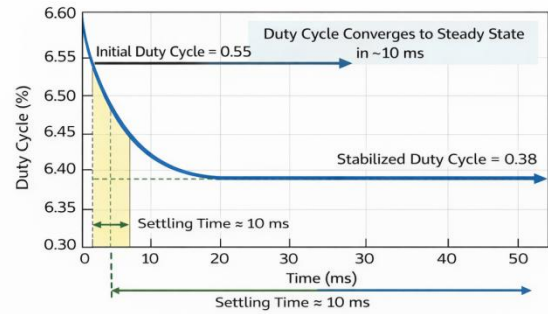
Figure 13: Duty Cycle Response of the FPGA-Based Fuzzy Logic MPPT Controller in the Solar Subsystem.
