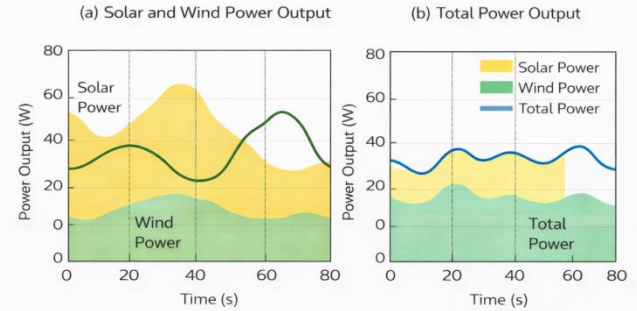
Figure 17: Complementary Solar and Wind Power Output Under Varying Conditions.
