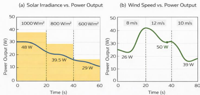
Figure 16: System Response to Varying Solar Irradiance (a) and Varying Wind Speed (b).
