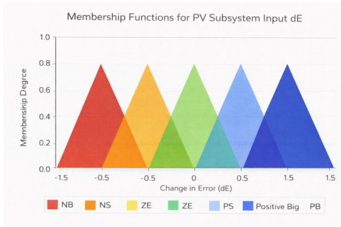
Figure 5. Membership Functions for PV Subsystem Input dE
