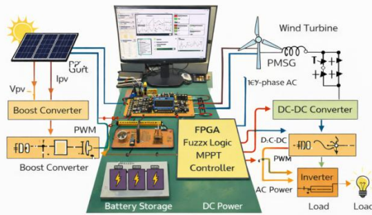
Figure 20: Experimental Setup of the FPGA-Based Fuzzy Logic MPPT Hybrid System
