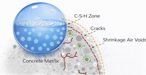
Figure 11: Schematic of the Transitional Zone Between Lightweight Water-Absorbent Polymer Beads and Concrete Matrix
