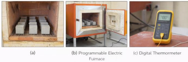
Figure 3: Fire Exposure Setup
