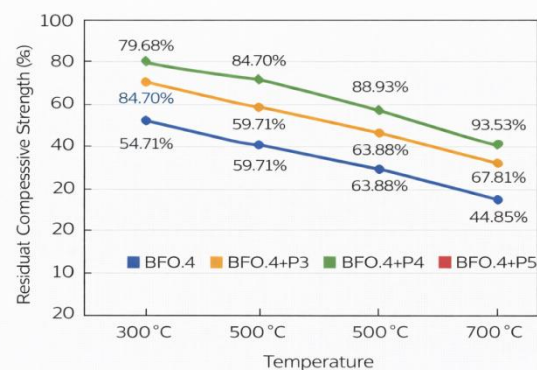
Figure 7: Residual Compressive Strength After Fire exposure
