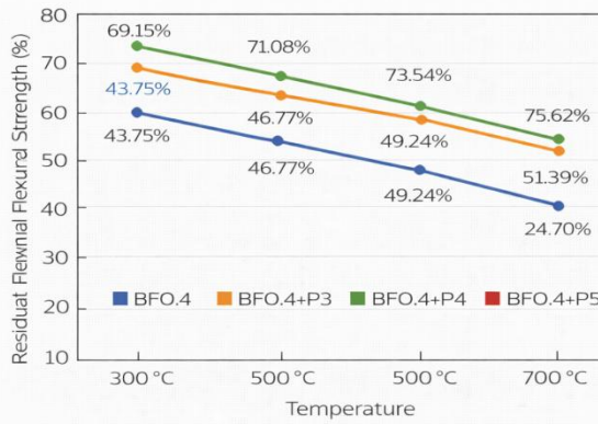
Figure 9: Residual Flexural Strength After Fire exposure
