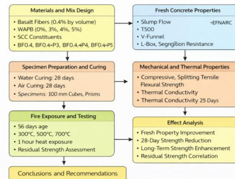
Figure 1: Research Methodology for the Effect of WAPB on Basalt Fiber-Reinforced SCC Exposed to Elevated Temperatures
