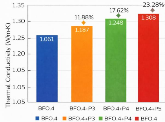
Figure 5: Thermal Conductivity of SCC Mixtures at 28 Days
